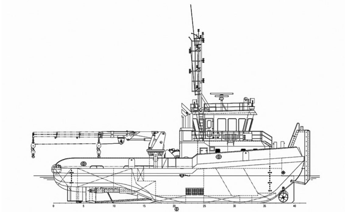
SIDE VIEW
