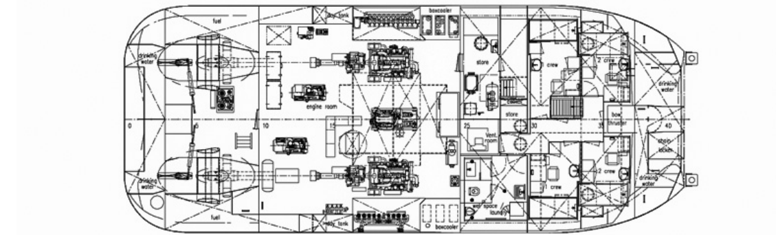
TOP VIEW DECK LEVEL
